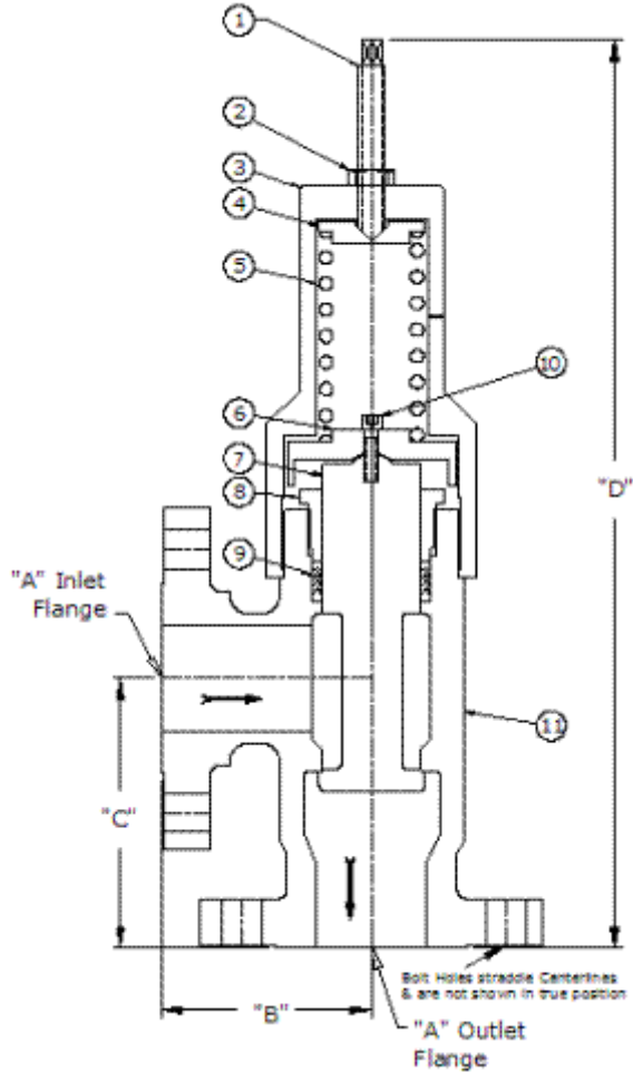
Model PRH-04-300#Fig 300# ANSI Flanged connections
