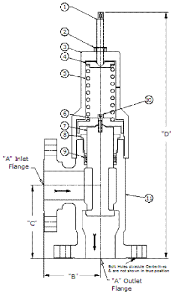
Model PRH-04-2500#Fig 2500# ANSI Flanged connections
